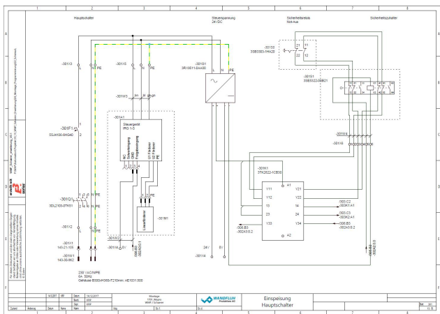
Example electrical diagram
