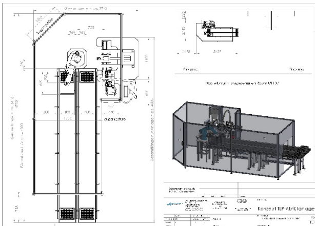
Massplan
